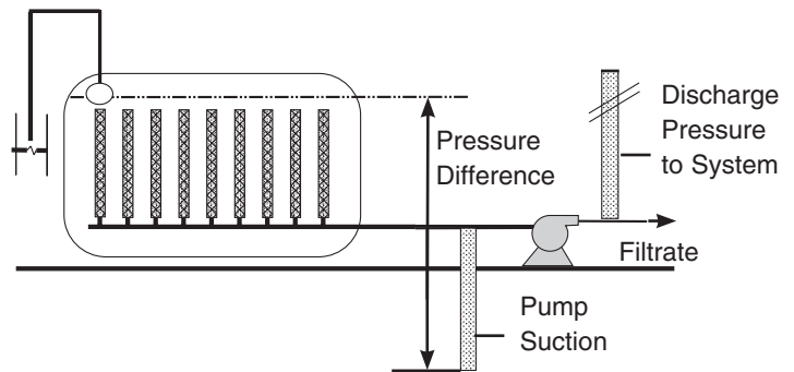
Figure 3-B Vacuum Filter
