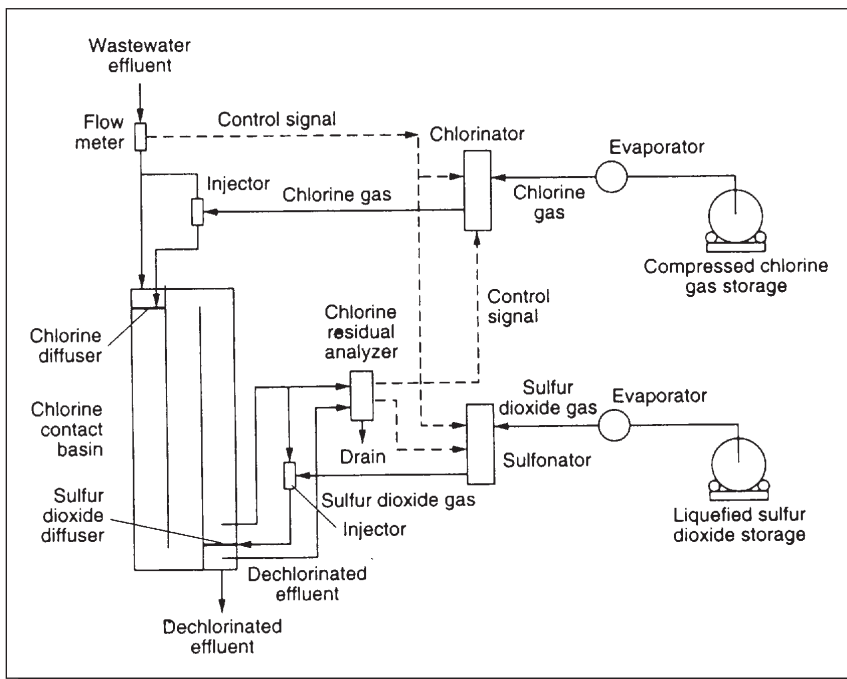
Figure 1: A compound-loop control system for chlorination with liquid chlorine and dechlorination with sulfur dioxide Source: Crites and Tchobanoglous (1998), used with permission from The McGraw-Hill Companies
