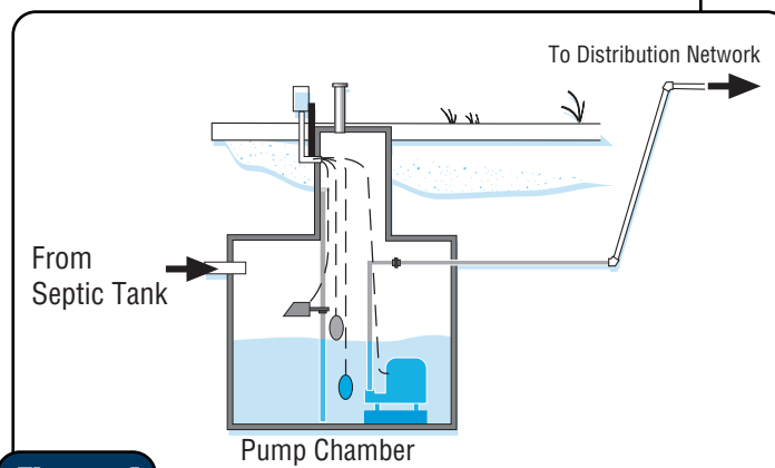
Figure 4 Typical pump system.
